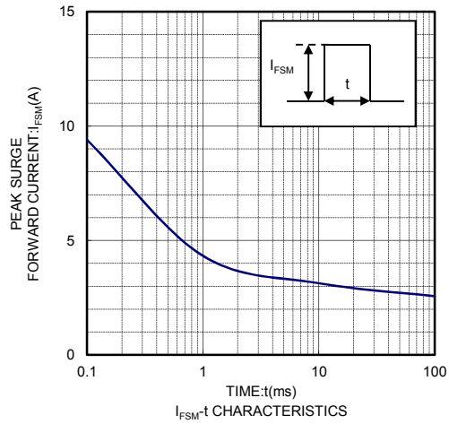
IFSM-t CHARACTERISTICS
