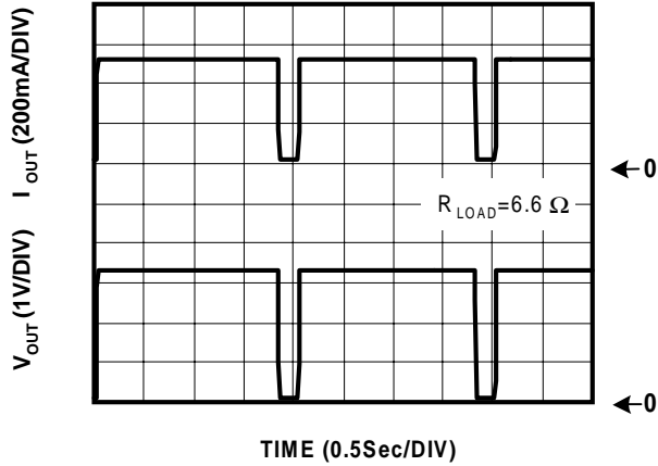
Overtemperature Shutdown
