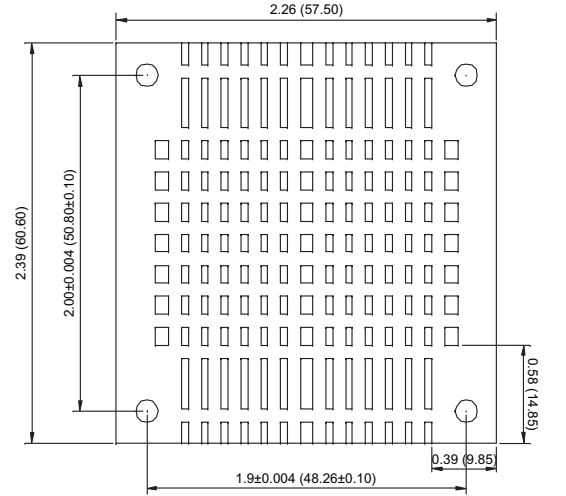
Heatsink Option (Suffix "HS")
