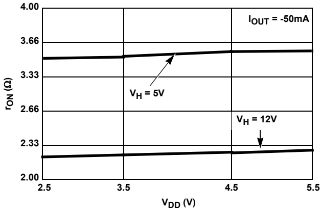
FIGURE 5. r_{ON} vs V_{DD} VOLTAGE (SOURCING CURRENT)
