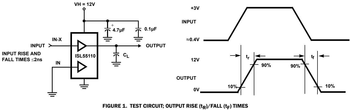
FIGURE 1. TEST CIRCUIT; OUTPUT RISE ( t_R )/FALL ( t_F ) TIMES
