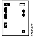
Figure 2. Metallization Diagram
