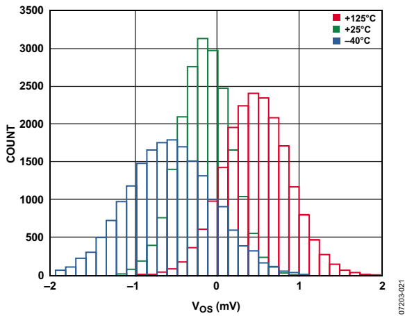
Figure 23. Offset Distribution
