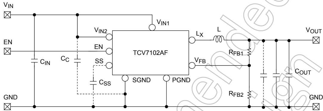
Figure 1 TCV7102AF Application Circuit Example
