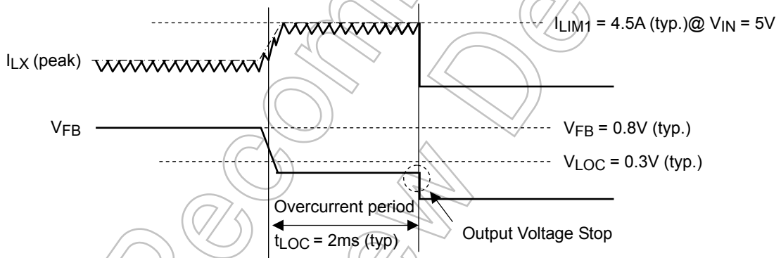
Figure 4 Overcurrent Operation
