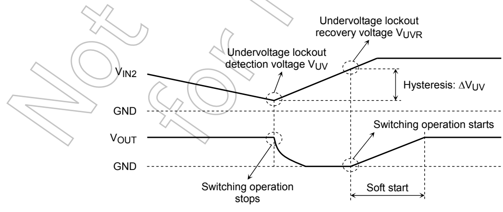
Figure 4 Undervoltage Lockout Operation
