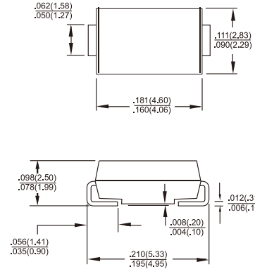
Dimensions in inches and (millimeters) Marking Diagram
