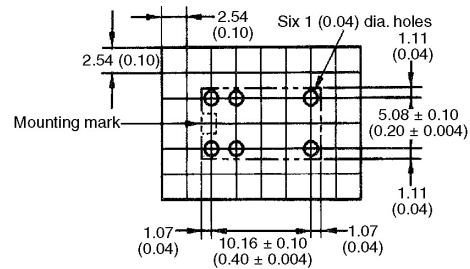
Mounting holes (bottom view)
