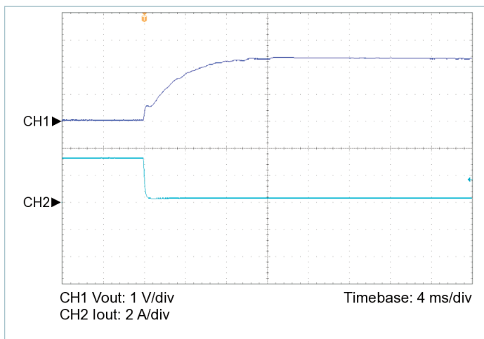
Figure 7 — 100% to 10% load transient response, V_{IN} = 30\text{ V} , nominal trim, C_{OUT\_EXT} = 220\ \mu\text{F}
