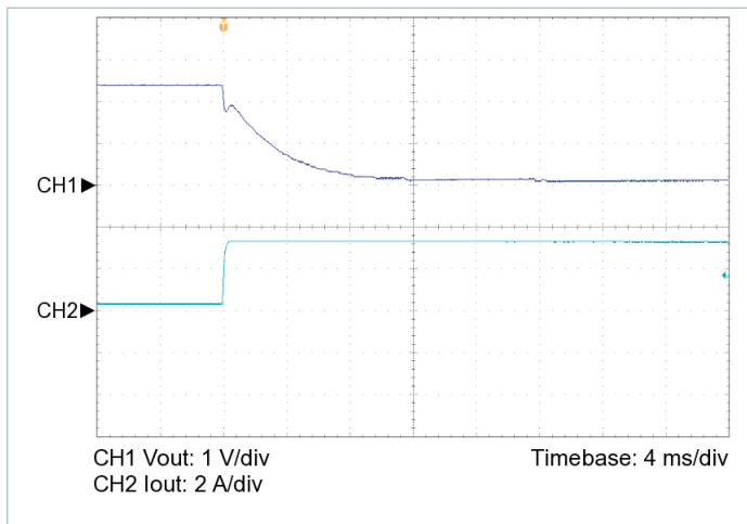
Figure 8 — 10% to 100% load transient response, V_{IN} = 30\text{ V} , nominal trim, C_{OUT\_EXT} = 220\ \mu\text{F}
