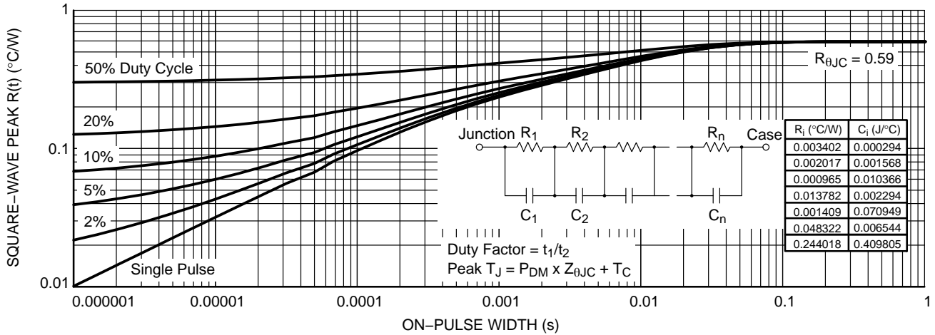
Figure 20. Diode Die Self-heating Square-wave Duty Cycle Transient Thermal Response
