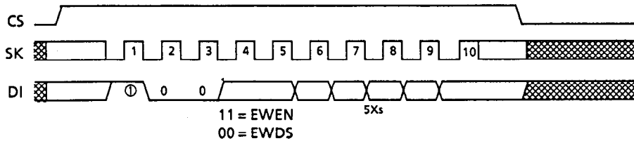
Figure 25 EWEN/EWDS Timing (S-29230A)
