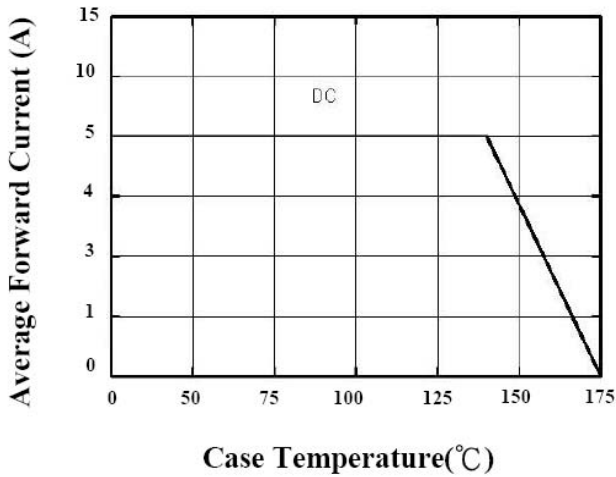
Fig.1- Forward Current
