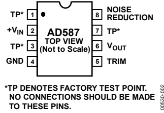
Figure 2. Pin Configuration
