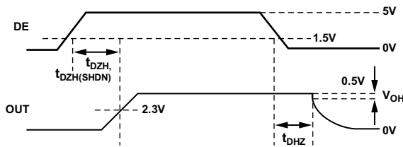
Figure 21. Driver Enable and Disable Times ( t_{DZH} , t_{DZH} , t_{DZH(SHDN)} )
