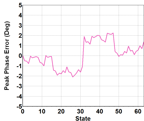
Peak Phase Error versus state @ 5.5GHz (wafer measurement)
