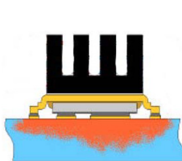
⑦ Mounted to a PCB with a thin gap filler and heat sink. (still air)
