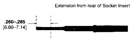
Round Solder-Post Socket (Loose Piece) Part Number 205544-1 — .031 [0.79] Dia. Tail Part Number 205544-2 — .023 [0.58] Dia. Tail
