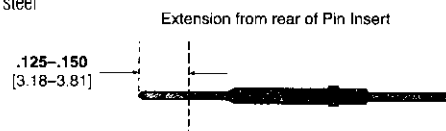
Round Solder-Post Pin Part Number 205753-2 (Loose Piece)
