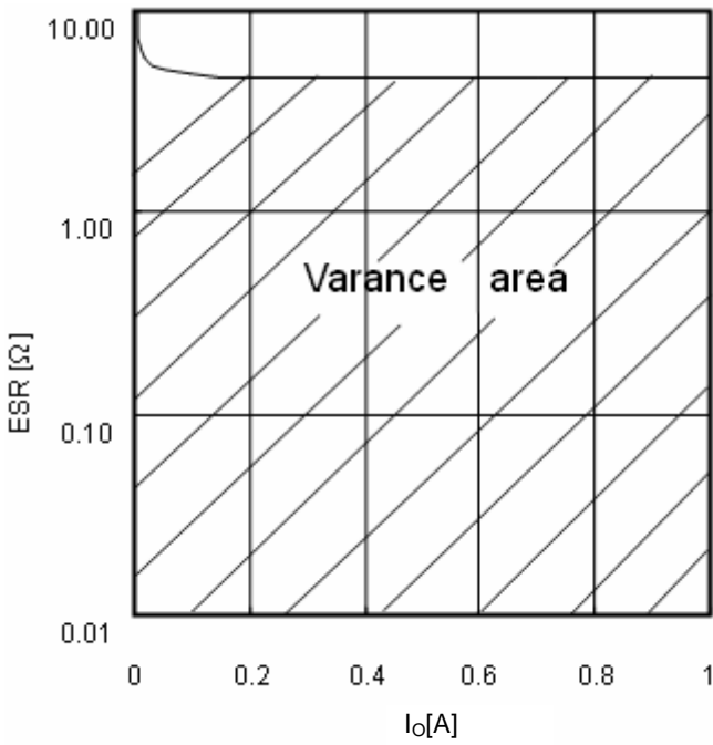
Fig.18 ESR condencer
