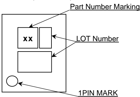
HVSOF6(TOP VIEW)
