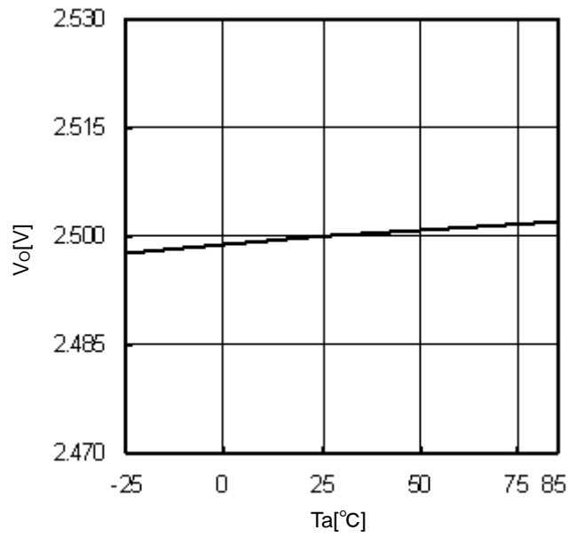
Fig.10 T<sub>a</sub>-V<sub>o</sub> (I<sub>o</sub>=0A)
