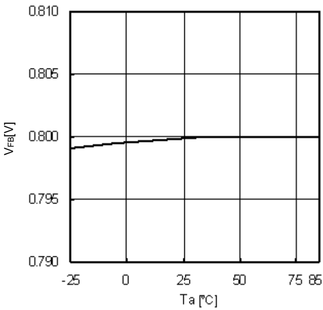
Fig.9 T<sub>a</sub>-V<sub>FB</sub>
