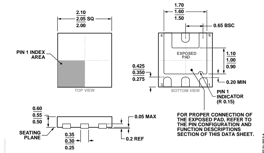
Figure 47. 6-Lead Lead Frame Chip Scale Package [LFCSP_UD] 2 mm × 2 mm Body, Ultrathin, Dual Lead (CP-6-7) Dimensions shown in millimeters
