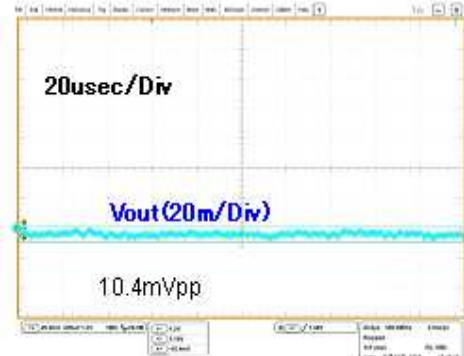
Figure 48. Output Ripple 4 ( V_{CC}=12V , I_o=170mA )
