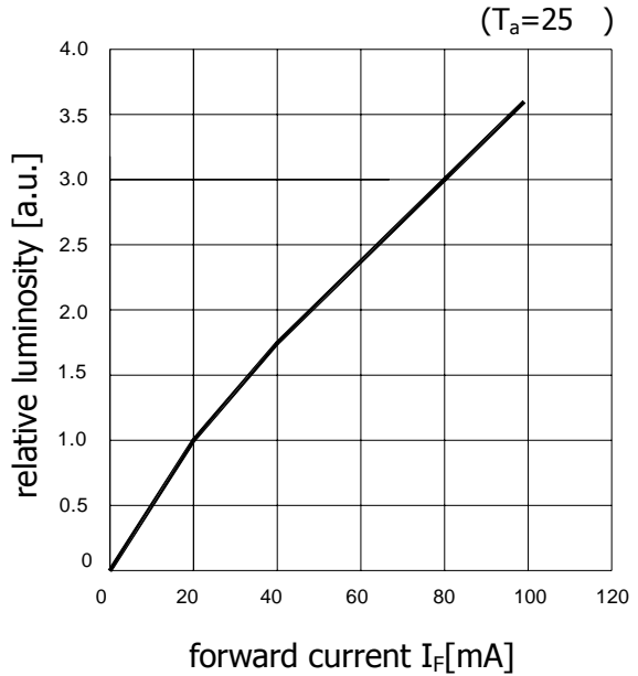
(2) forward current vs. relative luminosity
