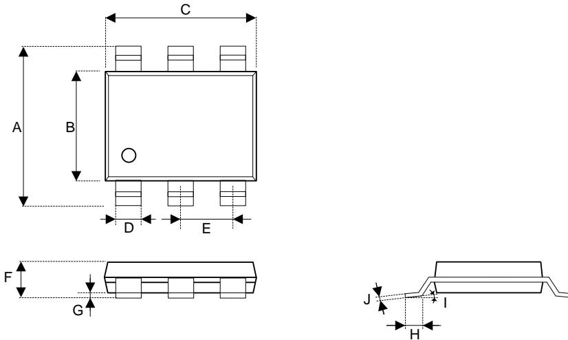
Figure 9.1 TSOT23-6 Packaging 1
