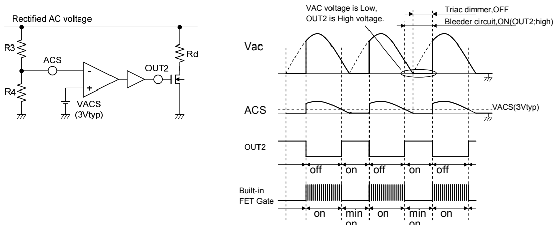
Waveforms diagram
