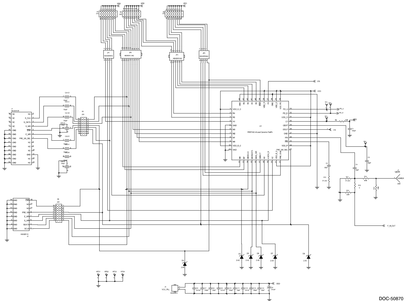
Figure 20. Evaluation Board Schematic
