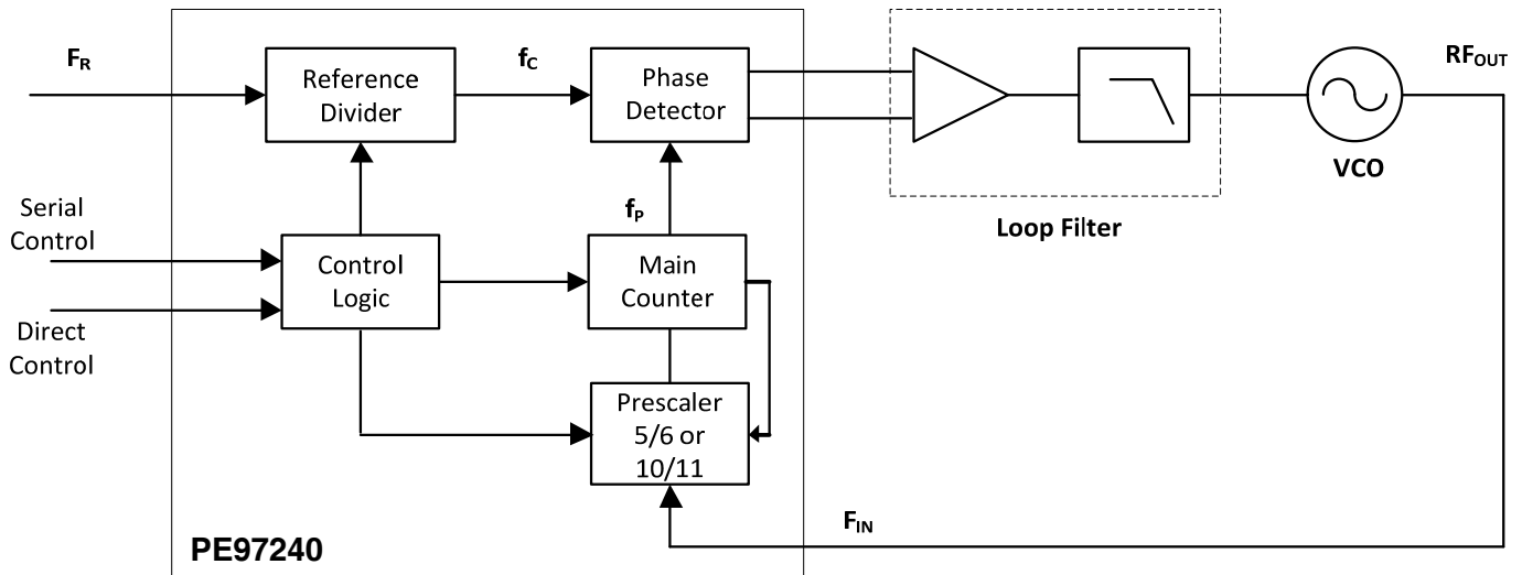
Figure 1. Functional Diagram
