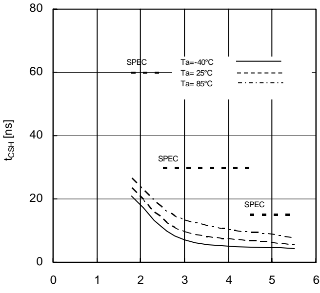
Figure 25. CSB Hold Time vs Supply Voltage
