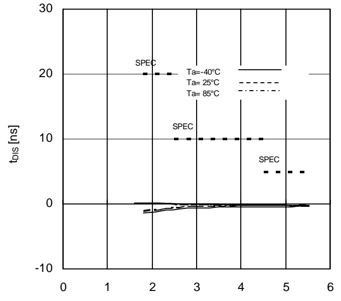
Figure 26. SI Setup Time vs Supply Voltage
