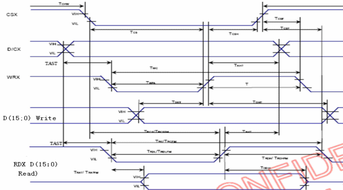
Fig 7.7.1.1 Parallel Interface characteristics (6050-Series MCU)
