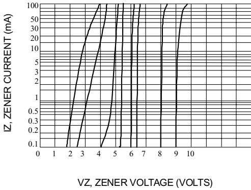
Fig. 6-VZ = 3.9 THRU 10 VOLTS
