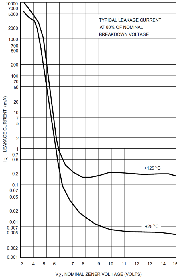
Figure 8. Typical Leakage Current
