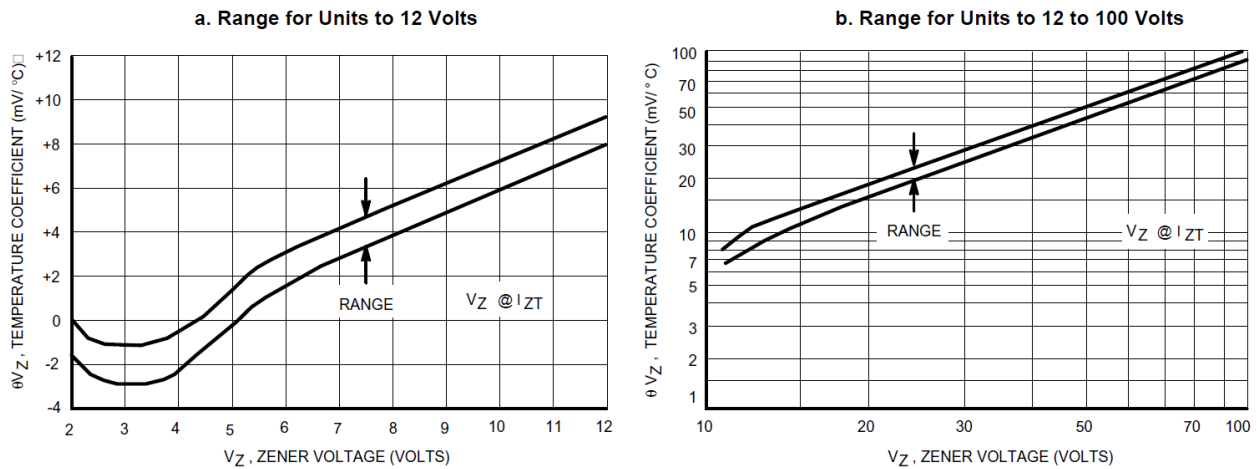
Figure 2. Temperature Coefficients
