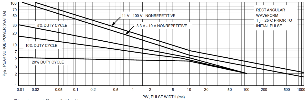
This graph represents 90 percentile data points. For worst case design characteristics, multiply surge power by 2/3.
