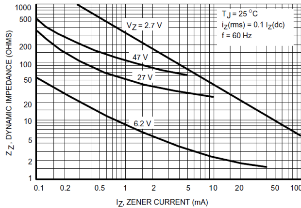
Figure 6. Effect of Zener Current on Zener Impedance
