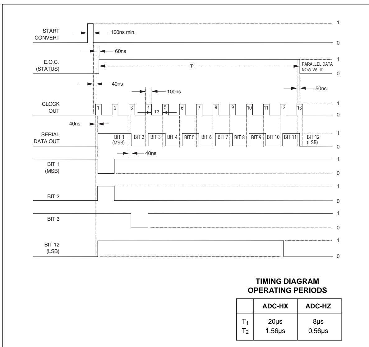
TIMING DIAGRAM FOR ADC-HX, ADC-HZ OUTPUT: 101010101010
