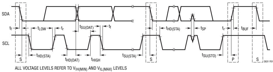
Figure 1. Serial Interface Timing
