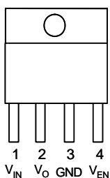
TO-220F-4
