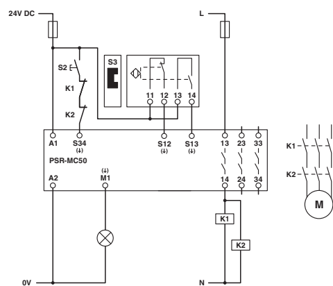
Circuit diagram
