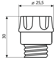
Fuse carrier/cap
