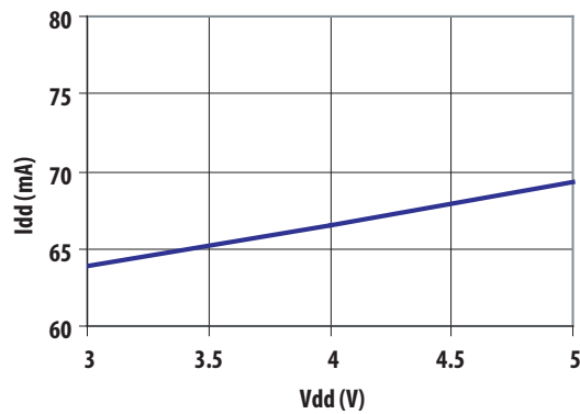
Figure 11. Idd over Vdd
