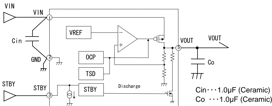
Fig. 2 Block Diagrams
