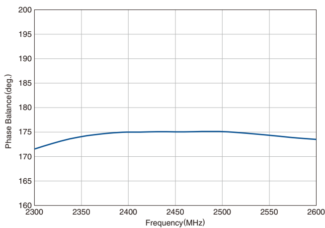
PHASE BALANCE
