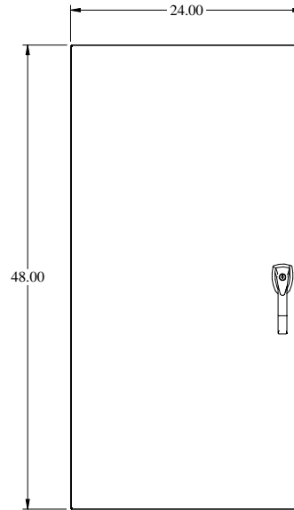
FRONT VIEW
