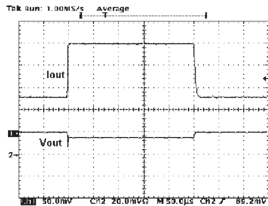
Figure 27 : Load Transient
