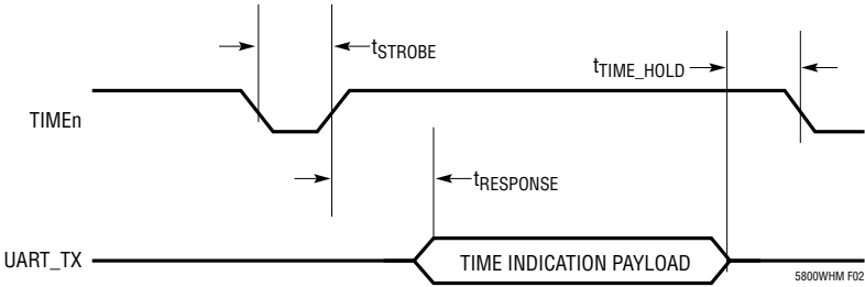
Figure 2. Timestamp Timing
