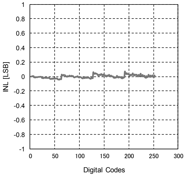
Fig.45 VCOM INL
