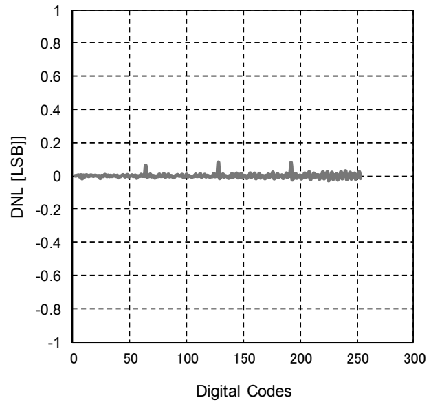
Fig.46 VCOM DNL
