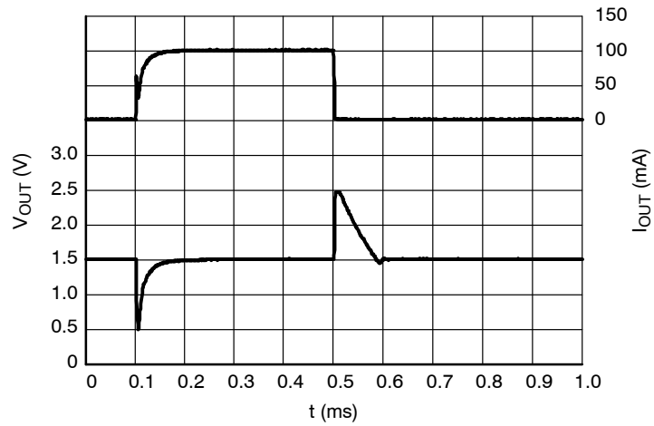
Figure 29. Load Transients, 1.5 V Version, I OUT = 1 – 100 mA, t R = t F = 0.5 μs, V IN = 2.5 V
