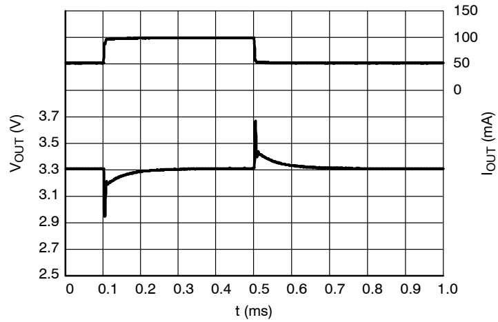
Figure 28. Load Transients, 3.3 V Version, I OUT = 50 – 100 mA, t R = t F = 0.5 μs, V IN = 4.3 V
