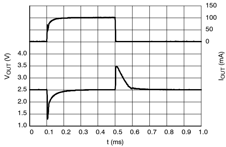
Figure 30. Load Transients, 2.5 V Version, I OUT = 1 – 100 mA, t R = t F = 0.5 μs, V IN = 3.5 V
