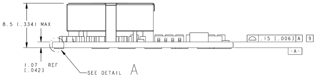
Side View
