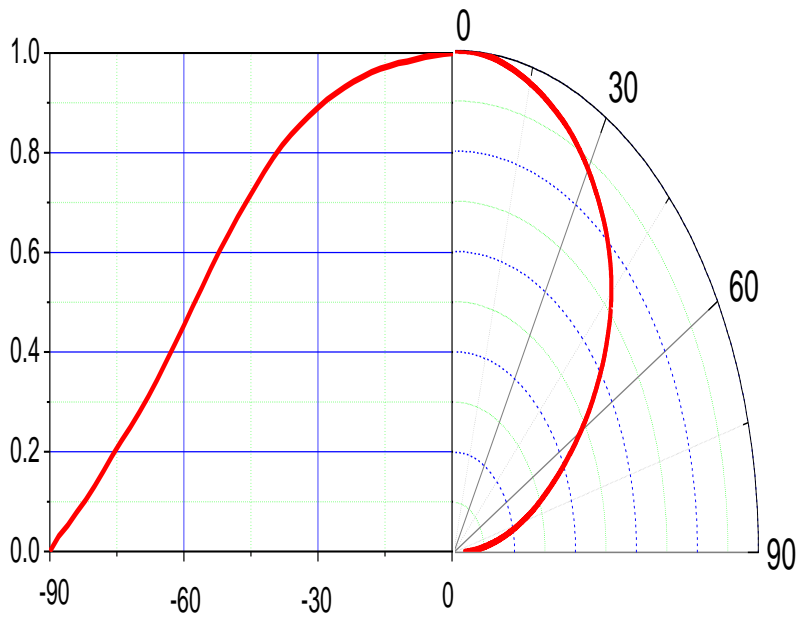
Fig 2. Viewing Angle Distribution, I_F = 140\text{mA}
