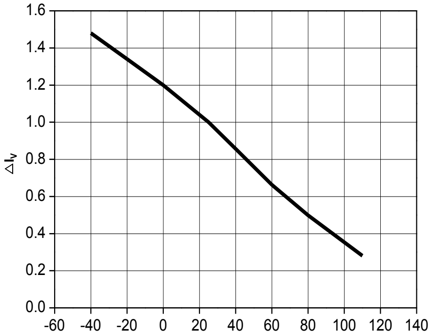
Fig 6. Relative Light Output vs. Junction Temperature, I_F = 140\text{mA}
