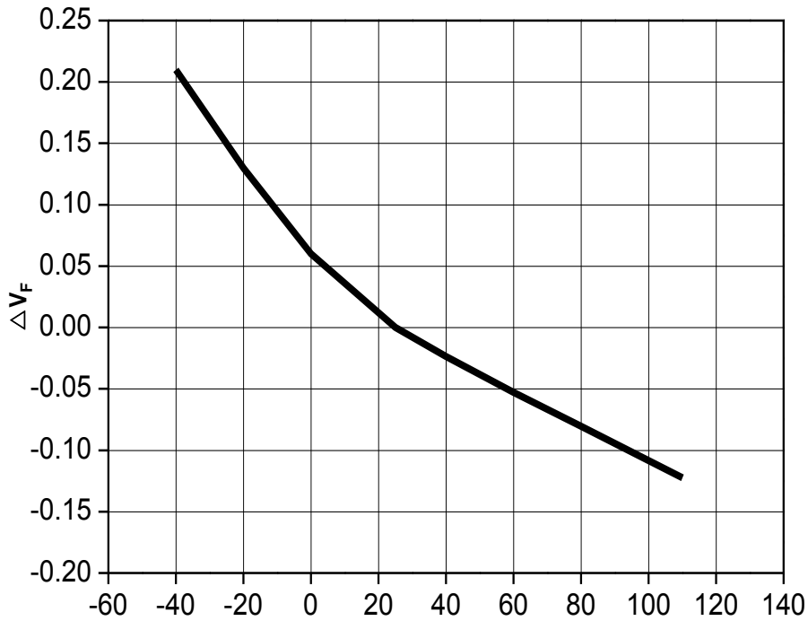
Fig 7. Junction Temperature vs. Forward Voltage shift, I_F = 140\text{mA}
