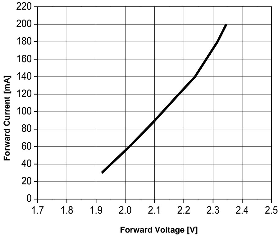
Fig 3. Forward Voltage vs. Forward Current, T_a = 25^\circ\text{C}
