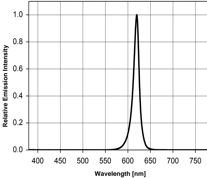
Fig 1. Color Spectrum, I_F = 140\text{mA} , T_a = 25^\circ\text{C} , RH30%
