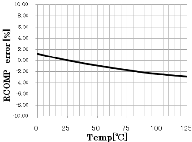
Figure 31, RCOMP Error
