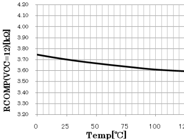
Figure 30, RCOMP (VCC=12)
