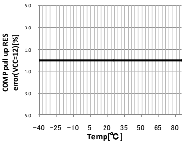
Figure 29, COMP Pull-up RES Error (VCC=12)
