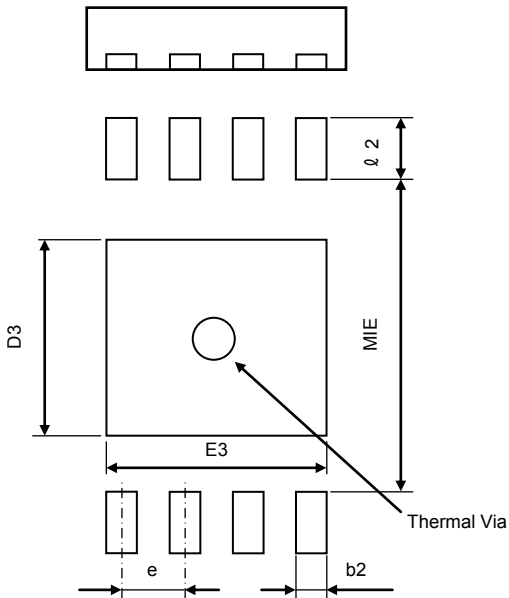
VSON008X2030
