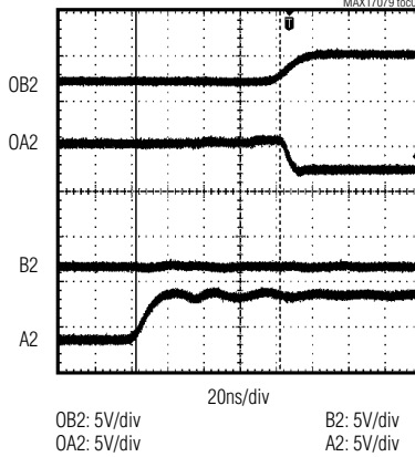
PROPAGATION DELAY (STATE 1 - STATE 2)
