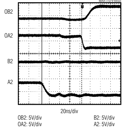
PROPAGATION DELAY (STATE 2 - STATE 3)
