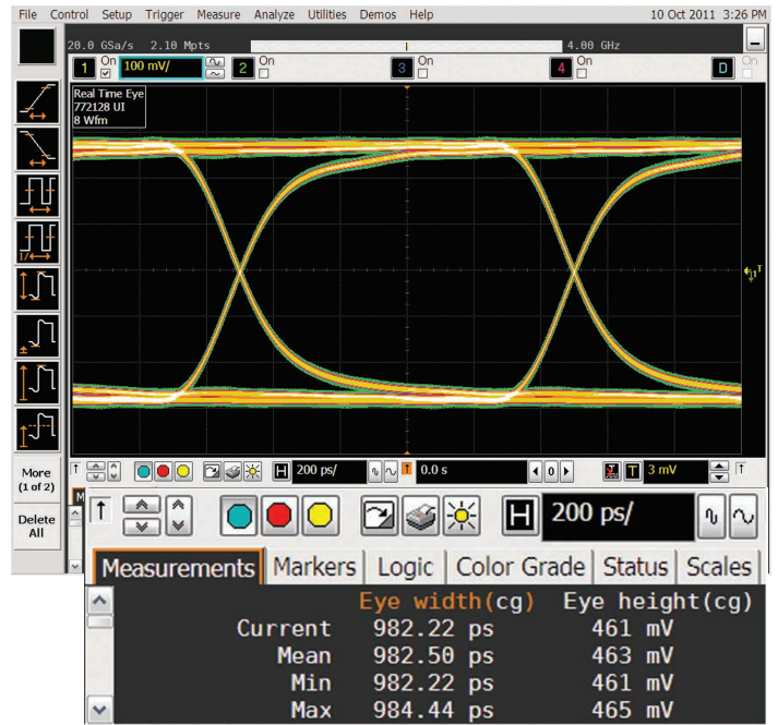
Figure 15. Real time eye with uncorrected cable loss
