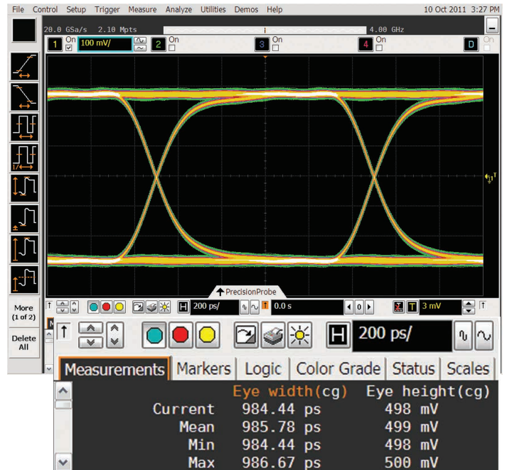
Figure 16. Real time eye with corrected cable using PrecisionProbe, notice that by correcting for cable loss there is a gain of 37mV in the eye height measurement!
