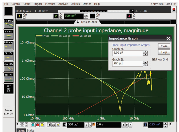
Figure 13. PrecisionProbe properly characterizes a 2 pF capacitor
