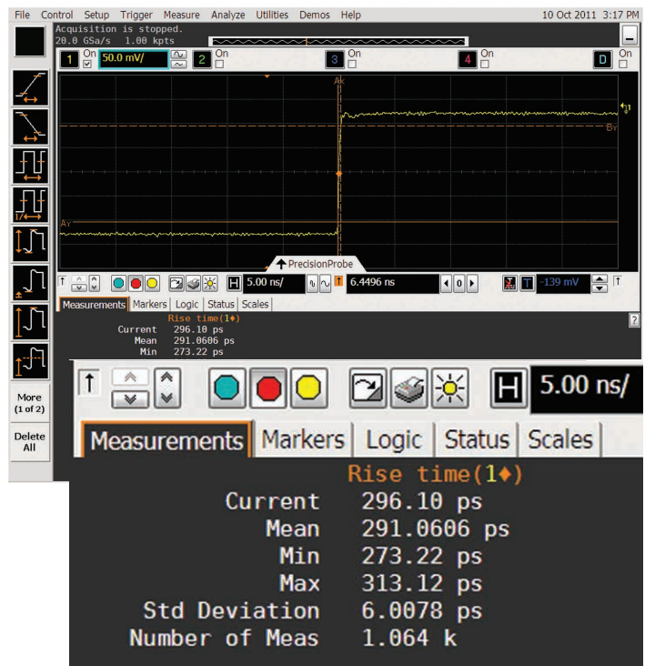
Figures 1 and 2. Cable loss degrades rise times and causes measurement non-repeatability. Figure 1 shows the rise time of a signal with a cable that’s loss is uncharacterized and not compensated. Figure 2 shows the same measurement with characterization and compensation. Notice the rise time is >15% faster and the measurement is nearly 50% more repeatable.
