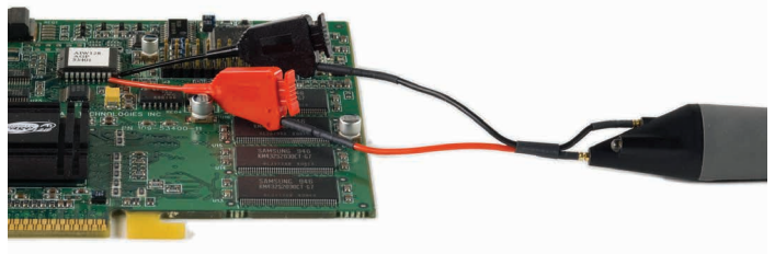
Figure 4. Image of custom probe
