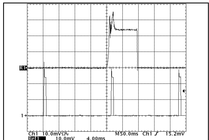
Figure 18: Load current ( 10\text{A}/\text{div} ) as a function of time when the converter attempts to turn on into a 10\ \text{m}\Omega short circuit. Top trace ( 4.0\text{ms}/\text{div} ) is an expansion of the on-time portion of the bottom trace.
